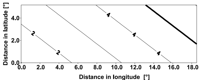
Fig. 2. Standard deviation (in nT) for the differences between observation points and geomagnetic observatory (or variation station) for geomagnetic activity level Kp = 0 .
