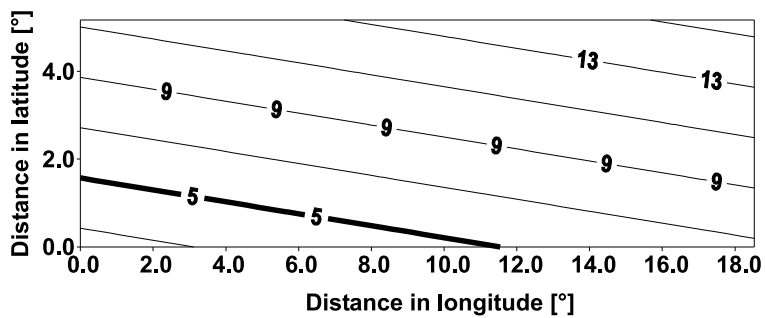
Fig. 4. Standard deviation (in nT) for the differences between observation points and geomagnetic observatory (or variation station) for geomagnetic activity level Kp = 5 .
