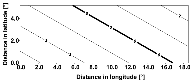
Fig. 3. Standard deviation (in nT) for the differences between observation points and geomagnetic observatory (or variation station) for geomagnetic activity level Kp = 4 .
