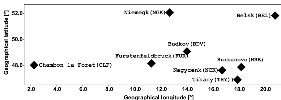
Fig 1. Distribution of geomagnetic observatories.
