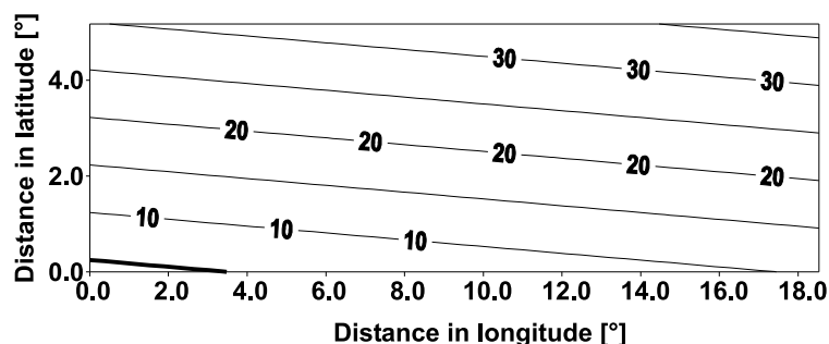
Fig. 5. Standard deviation (in nT) for the differences between observation points and geomagnetic observatory (or variation station) for geomagnetic activity level Kp = 7 .
